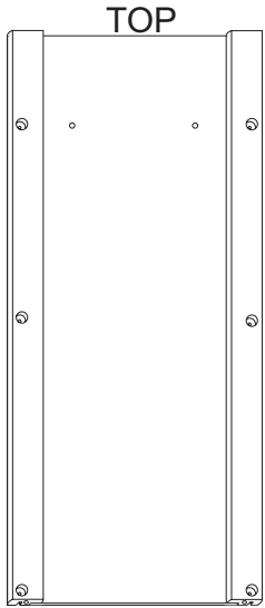
Handle Side Panel (1) P/N: SP/HDL - 51576
